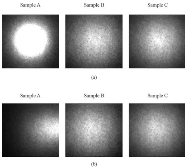
Figure 8. The energy diffused by the diffusing thin film detected with the measuring tool of experiment II. Energy incidence angle: (a) normal or 0^\circ ; (b) 60^\circ . Initially, the image captured was an 8-bit (256-level) greyscale. To show the effect of the diffuser on all the samples, the initial captured image has been matched to the next transformation. Sample A: the lowest level (0) corresponds to level 47; the highest level (255) corresponds to level 103. Sample B: the lowest level (0) corresponds to level 47; the highest level (255) corresponds to level 63. Sample C: the lowest level (0) corresponds to level 47; the highest level (255) corresponds to level 93.
