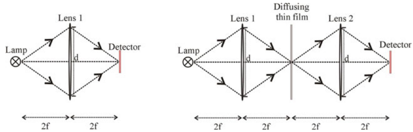
Figure 3. A transmitted energy measuring tool. This system works with an equivalent aperture number of N = 4 and a lateral magnification of m = -1 . (a) Initial energy detection without the diffusing thin-film contribution. (b) Detection of the proportion of energy transmitted by the diffusing thin film.
