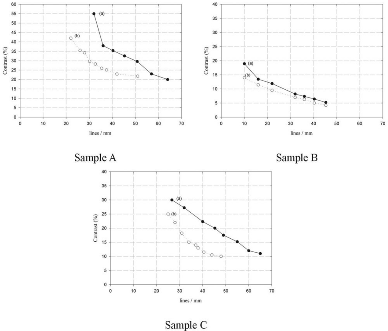
Figure 10. The MTF for the three samples evaluated. Incident energy angle: (a) normal or 0° (continuous curve); (b) 60° (dashed curve).
