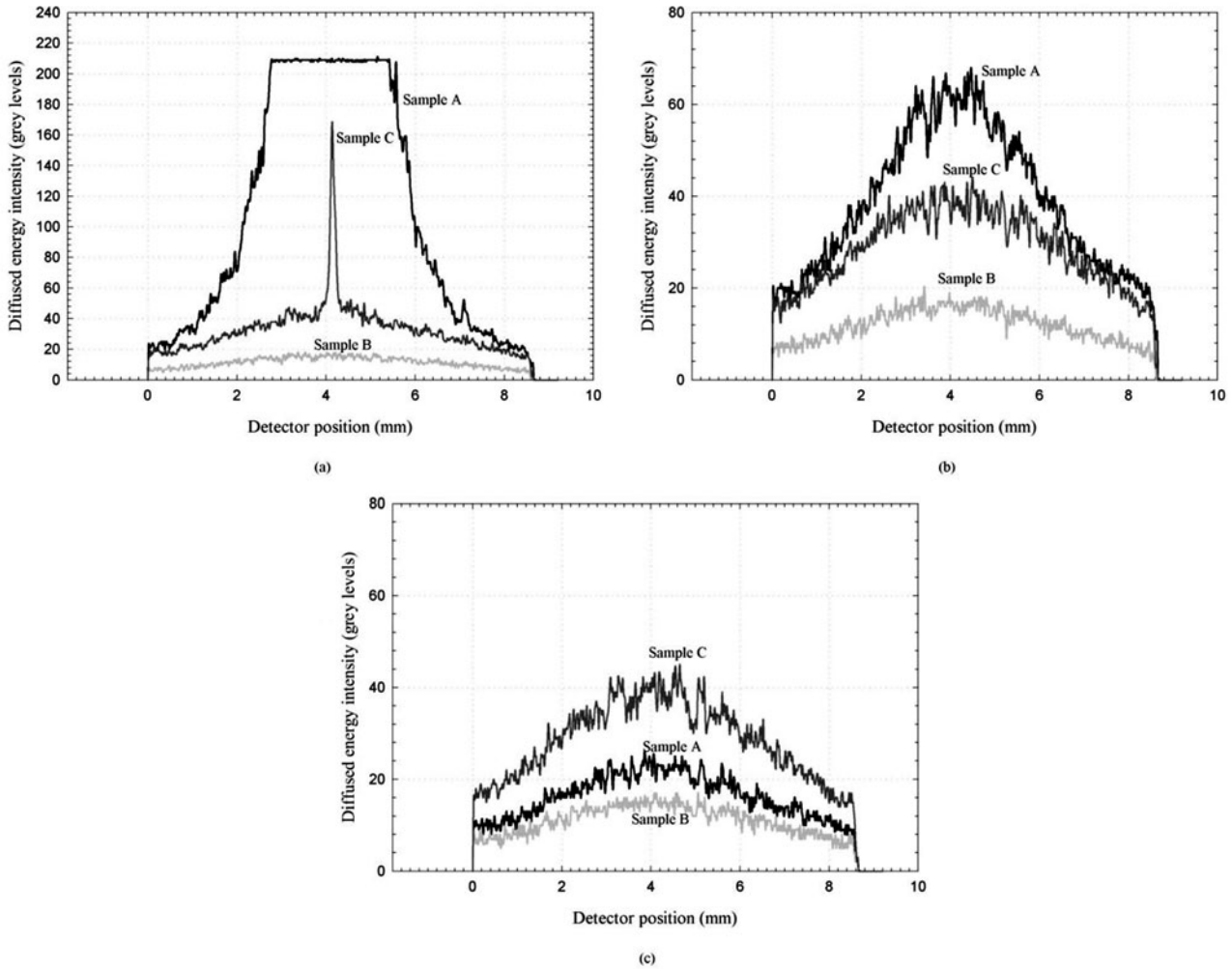
Figure 9. A cut of the diffused energy pattern. Incident energy angle: (a) normal or 0°; (b) 30°; (c) 60°. Sample A (black curve), sample B (beige curve), sample C (grey curve).
