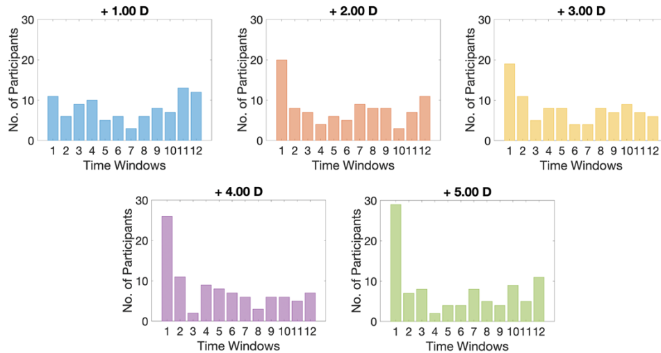
Fig. 6. Bar charts representing the number of participants who achieved the maximum relaxation of accommodation in each time window.
