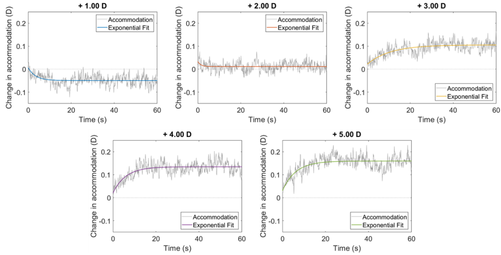
Fig. 4. Exponential fit to the accommodative responses to each lens.
