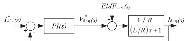
Fig. 2. Control scheme with the PI(s) controller, plant transfer function and the current, voltage and back EMF signals for the direct and quadrature axes.
