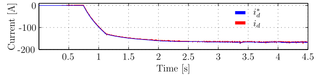
(a) d-axis current control.
