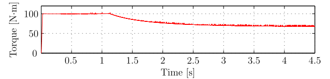
(c) SM-PMSM torque (estimated from the measured currents).
