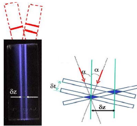
Fig 2. Propagation of two beams with \lambda=810\text{nm} overlapping within a \chi^{(2)} random nonlinear crystal. One of the beams is a unique short pulse, whereas the other beam is a sequence of two short sub-pulses. The two traces correspond to SHG light generated in the regions where pulse overlapping occurs. The trace width gives the pulse duration, whereas the trace separation gives the time separation between the two sub-pulses and thus can be used for absolute calibration of the measurement of the pulse width [12].
