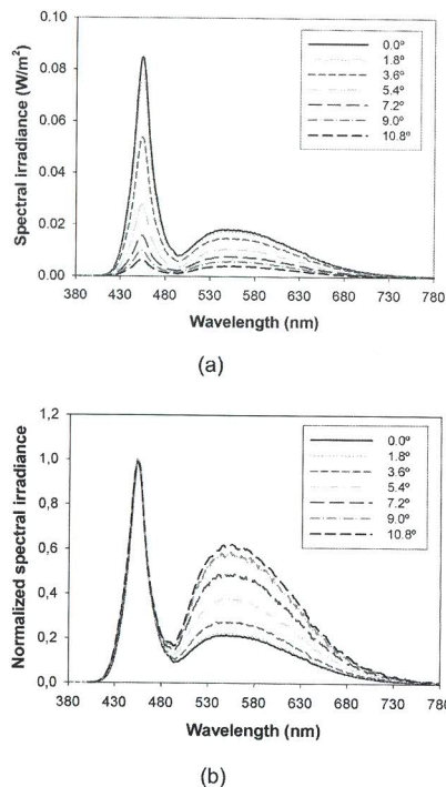
Figure 5. (a) Brand3 White 15° spectral irradiance [W/m 2 ] at different viewing angles and (b) normalized spectral irradiance.
