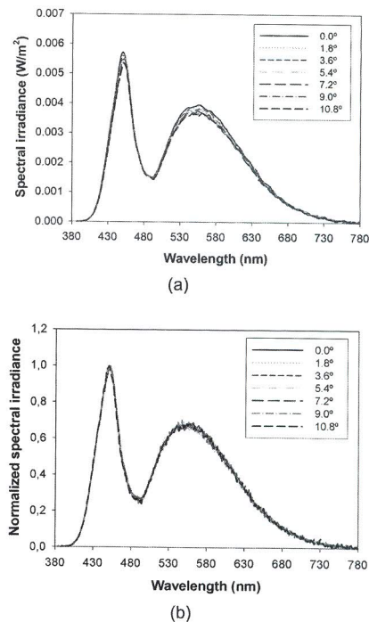
Figure 6. (a) Brand2 White 140° spectral irradiance [W/m 2 ] at different viewing angles and (b) normalized spectral irradiance.
