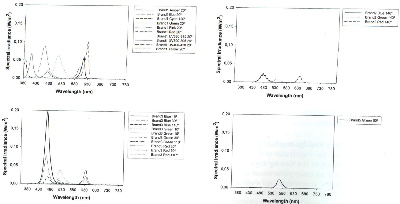
Figure 4. Single color LEDs spectral irradiance ( W/m^2 ) at a 0^\circ viewing angle.
