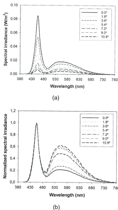
Figure 5. (a) Brand3 White 15° spectral irradiance ( \text{W}/\text{m}^2 ) at different viewing angles and (b) normalized spectral irradiance.
