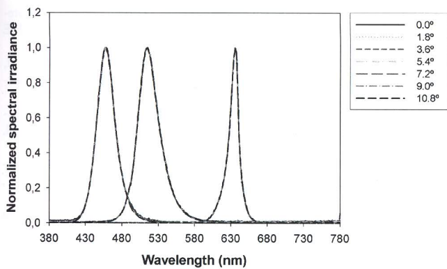
Figure 9. Normalized spectral irradiance of three single color LEDs (Brand1 Red LED 20°, Brand2 Green 20°, and Brand3 Blue 20°) at different viewing angles.
