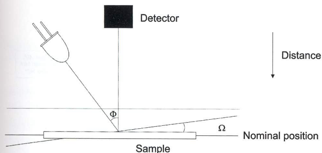
Figure 2. Schematic layout of the spectrophotometric system geometry (illumination angle [ \Phi = 45^\circ ]/measuring angle [ \Omega = 0^\circ ]).
