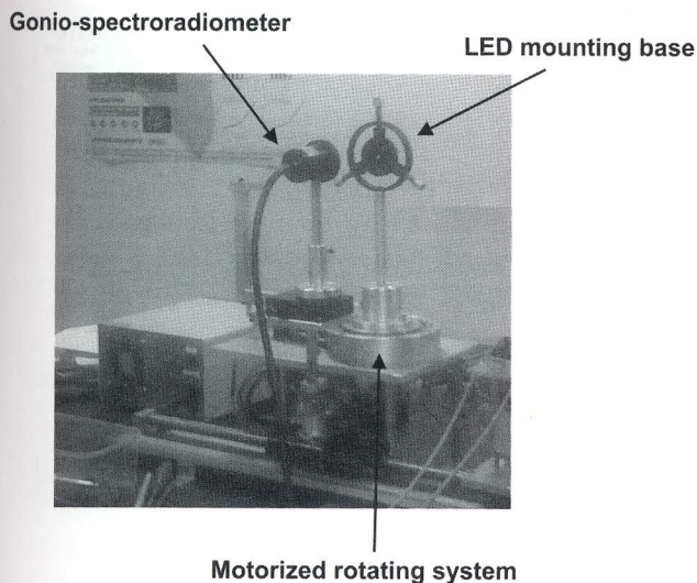
Figure 1. Experimental setup used for the spectral characterization of the LEDs at different angles.
