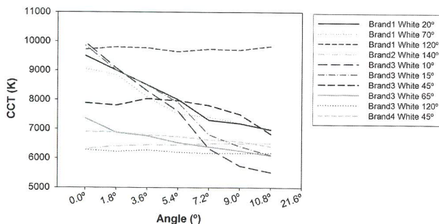
Figure 8. CCT of the white LEDs at different viewing angles.
