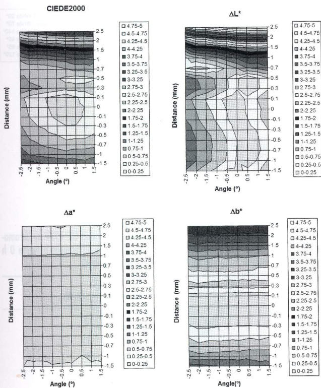
Figure 12. CIEDE2000 color differences between the measurements performed on a white ceramic tile surface at different angles and distances with respect to the nominal position. (a) CIEDE2000 color difference. (b) Same analysis expressed only in L^* terms. (c) In a^* terms and (d) in b^* terms.
