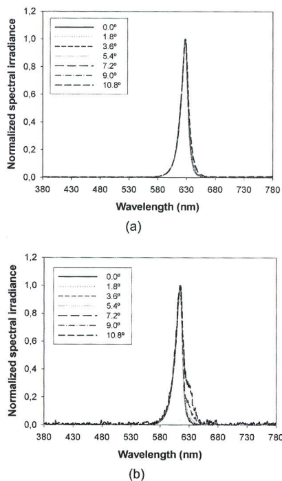
Figure 10. Normalized spectral irradiance of single color LEDs at different viewing angles: (a) Brand1 Red 20°, (b) Brand1 Amber 20°.
