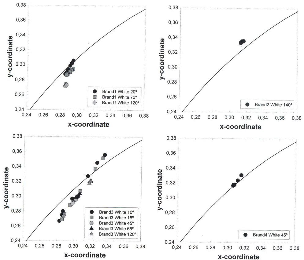
Figure 7. CIE 1931-xy chromaticity coordinates at different viewing angles for the white LEDs. The spectral locus is also shown in the chromaticity diagram.
