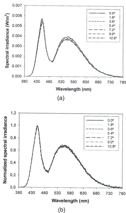
Figure 6. (a) Brand2 White 140° spectral irradiance ( \text{W}/\text{m}^2 ) at different viewing angles and (b) normalized spectral irradiance.
