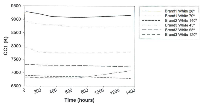
Figure 11. CCT of white LEDs with time of usage.
